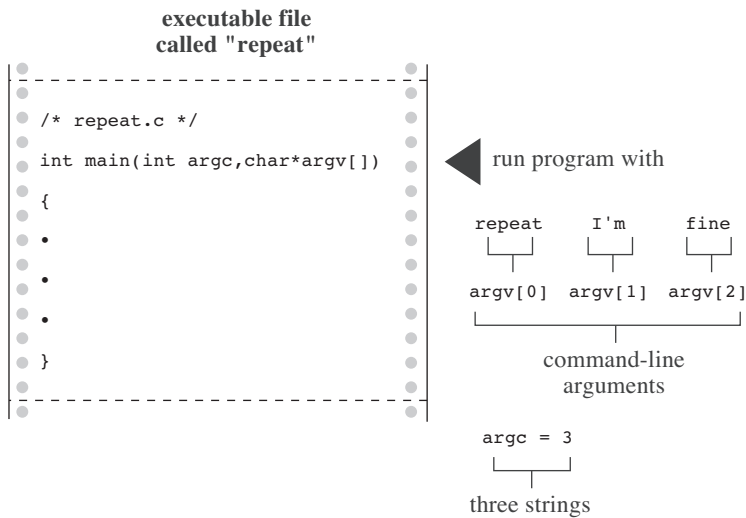
Figure 11.7 Command-line arguments.
